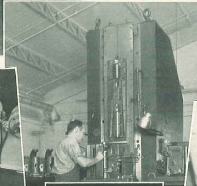
Modern high-production precision vertical broaching machine — one of many modern production units used in the manufacture of our power tools.
